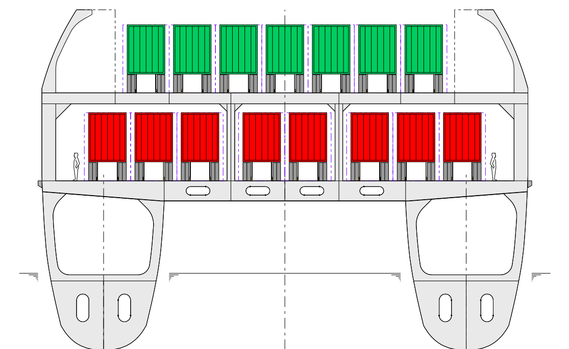
MIDSHIP SECTION
