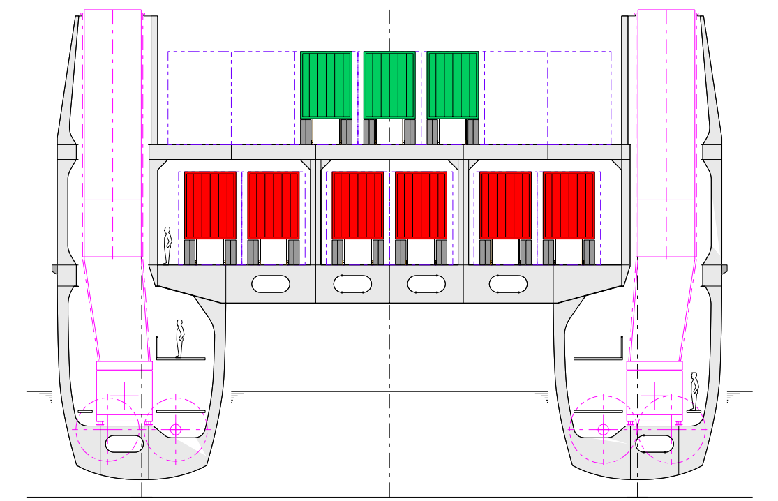
ENGINE ROOM SECTION
