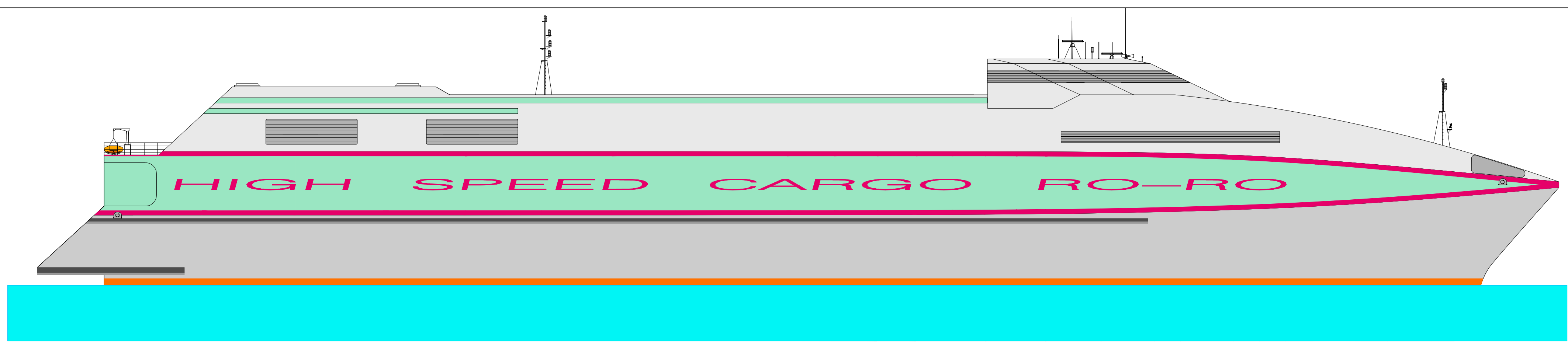
OUTBOARD PROFILE
